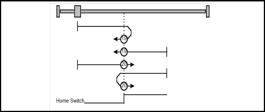
Figure 7-10 Homing on positive home switch
