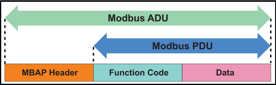
Figure 7-1 Modbus Data Structure
