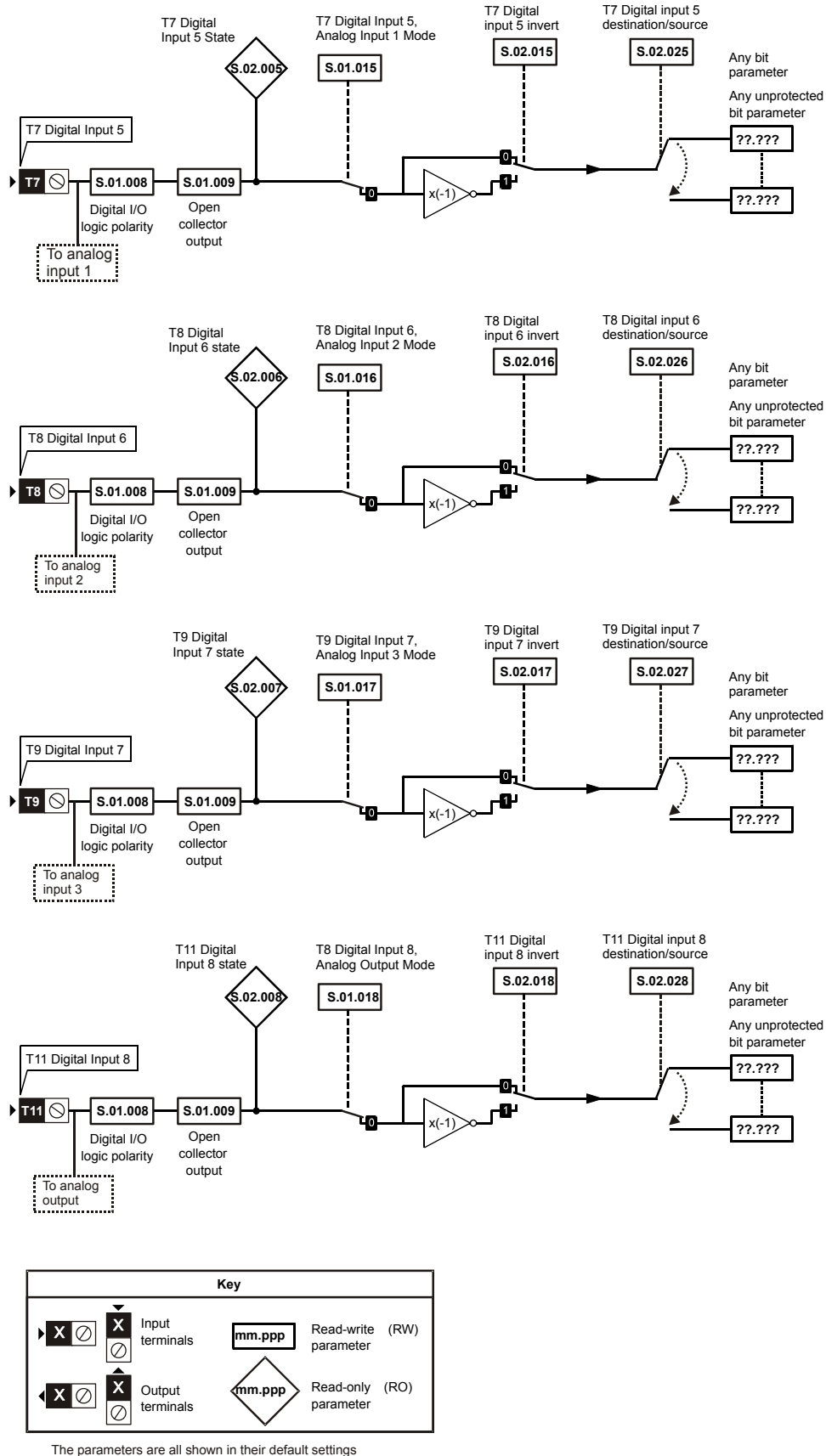
Figure 8-3 Digital input 5/6/7/8
