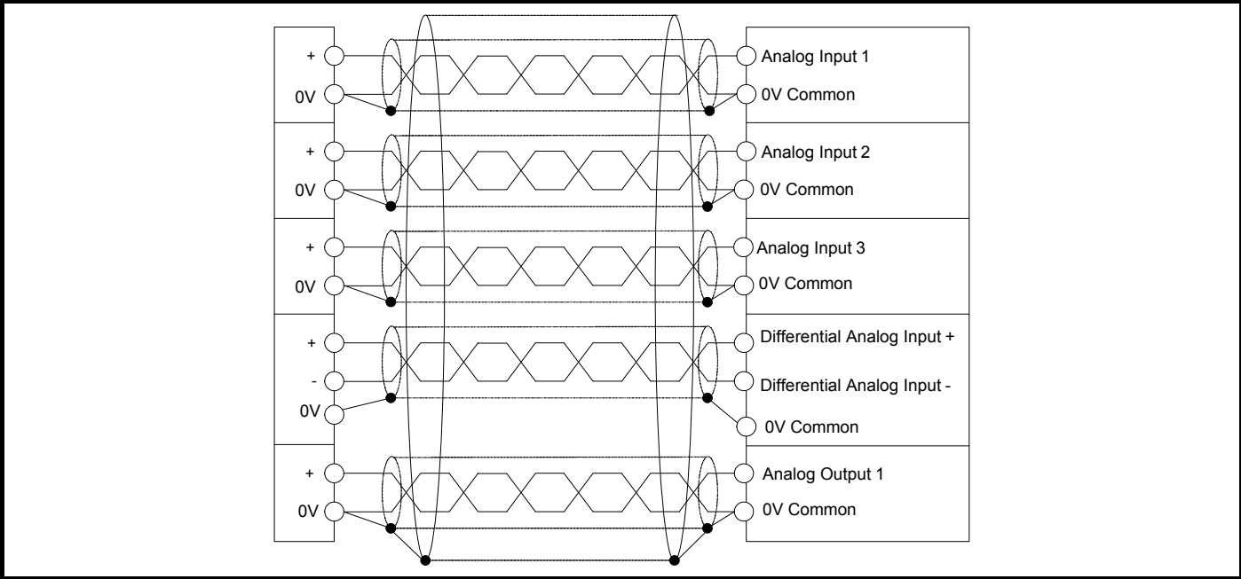
Figure 5-1 Shield connections
