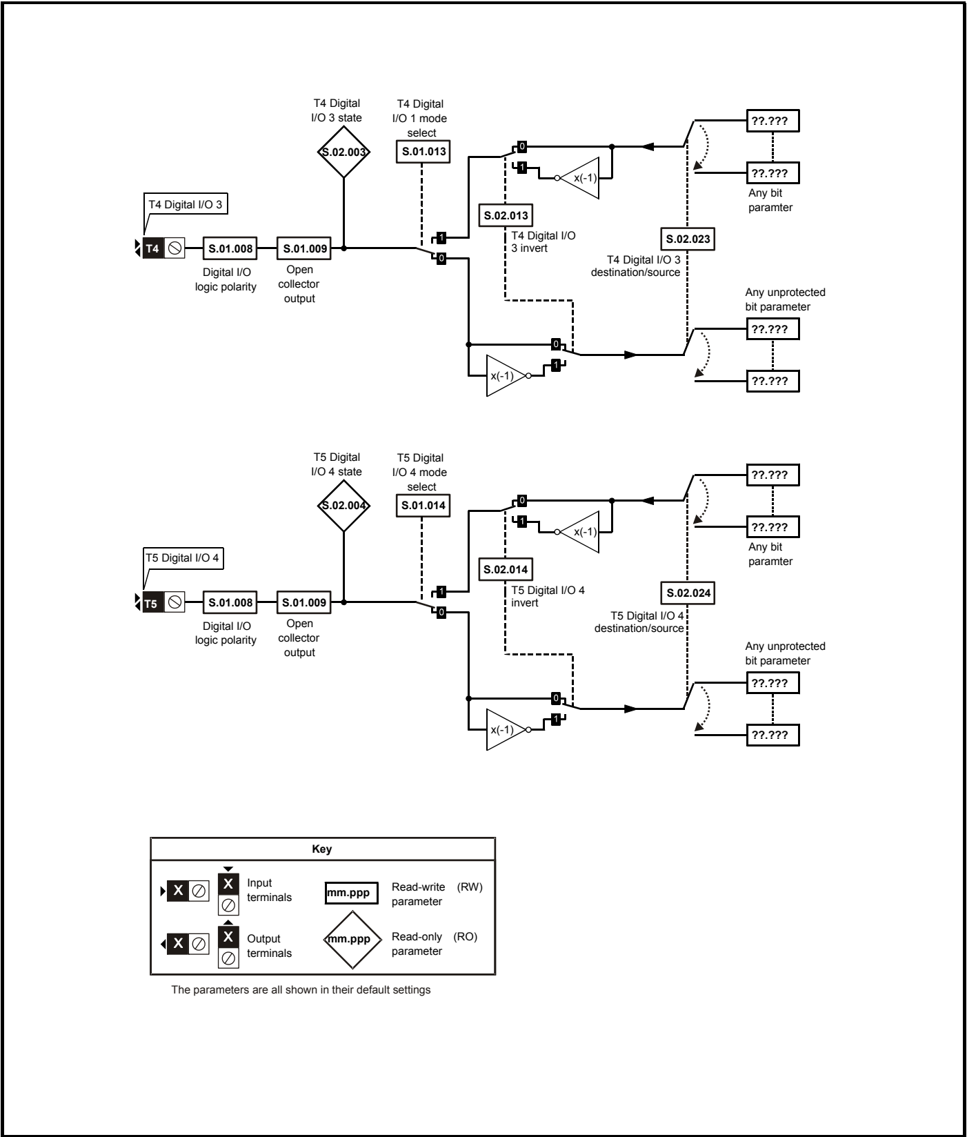
Figure 8-2 Digital I/O 3/4
