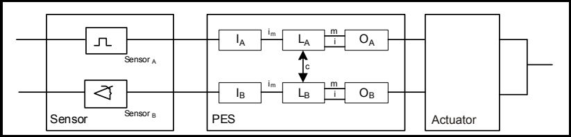
Figure 3-11 Sensors for speed and/or position recording
