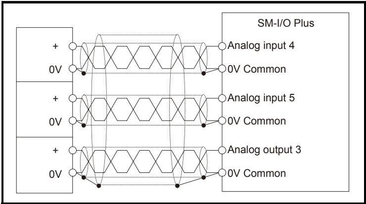
Figure 4-4 Shield connections
