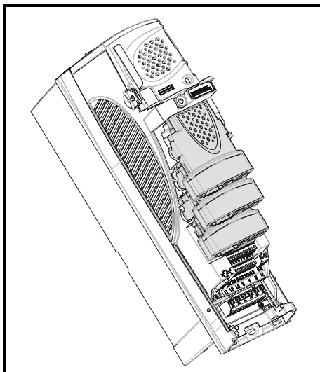
Figure 3-3 Unidrive SP with three Solutions Modules fitted
